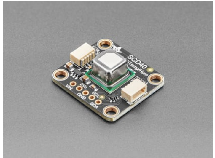
Adafruit SCD-40 - True CO2, Temperature and Humidity Sensor - STEMMA QT / Qwiic - STEMMA QT / Qwiic
