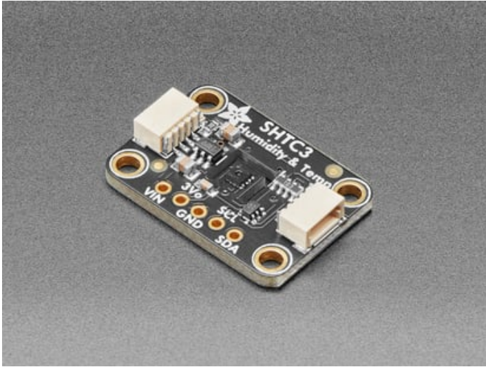
Adafruit Sensirion SHTC3 Temperature & Humidity Sensor - STEMMA QT / Qwiic - STEMMA QT / Qwiic
