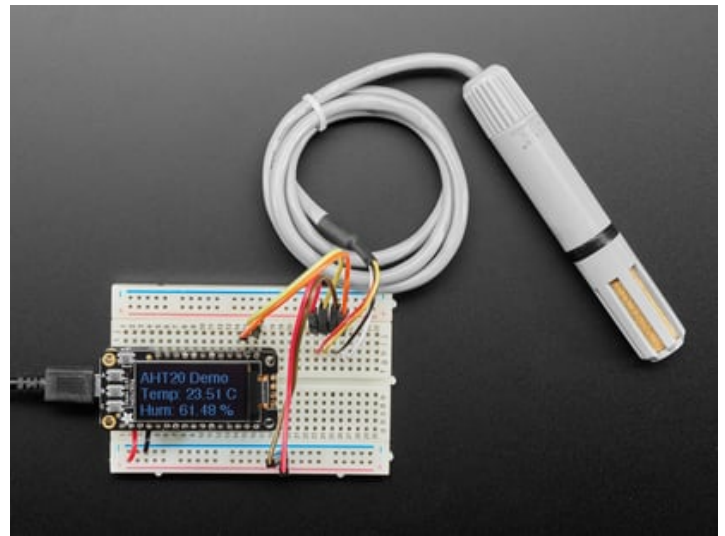
AM2315C - Encased I2C Temperature/Humidity Sensor
