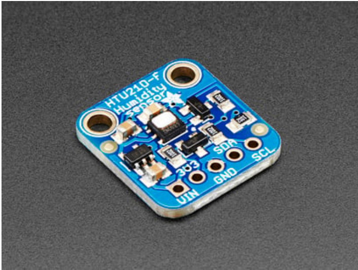
Adafruit HTU21D-F Temperature & Humidity Sensor Breakout Board - with or without Headers - with or without Headers
