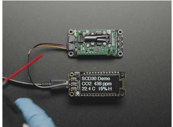
Adafruit SCD-30 - NDIR True CO2 Temperature and Humidity Sensor - STEMMA QT / Qwiic - STEMMA QT / Qwiic
