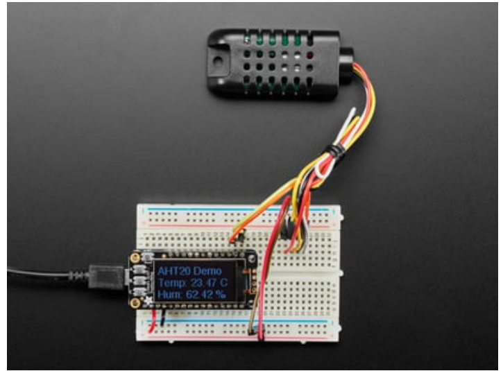
AM2301B - Wired Enclosed AHT20 - Temperature and Humidity Sensor
