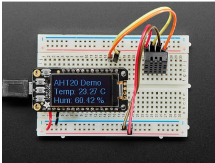
DHT20 - AHT20 Pin Module - I2C Temperature and Humidity Sensor
