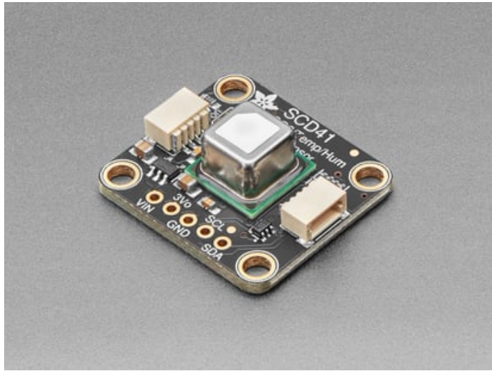
Adafruit SCD-41 - True CO2 Temperature and Humidity Sensor - STEMMA QT / Qwiic - STEMMA QT / Qwiic
